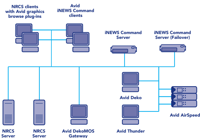
Avid iNEWS Command supports automated playback of multiple devices, including Avid Deko, Avid Thunder, and Avid AirSpeed systems, in an NRCS environment.
